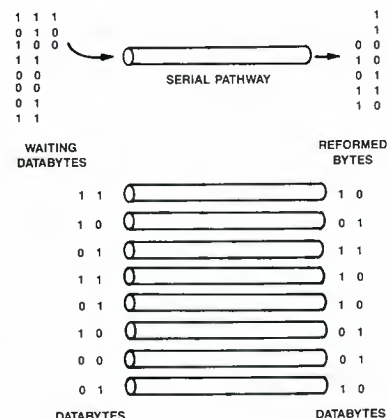
Figure 1. The serial RS-232 protocol must send data one bit at a time down the serial line; the parallel GPIB sends eight parallel bits at once. Additional technical differences allow the GPIB to be 260 times faster in some uses.
