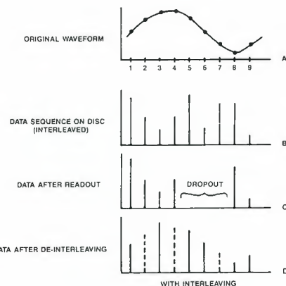
Figure 2. The recording process band-limits the audio. Therefore, you can assume there will be no abrupt changes between adjacent samples. This makes interpolation (the dashed lines shown here) fairly easy. Study the Nyquist theorem for more detailed explanation of why this is possible.
