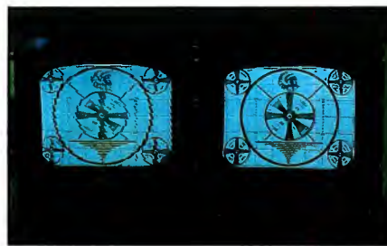
Early VTR engineers constantly had to cope with venetian blinding (shown at left), caused either by inadequate tip penetration or incorrect head spacing (quadrature error). (Courtesy of Ampex.)
